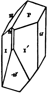
Hebronite, Maine.
